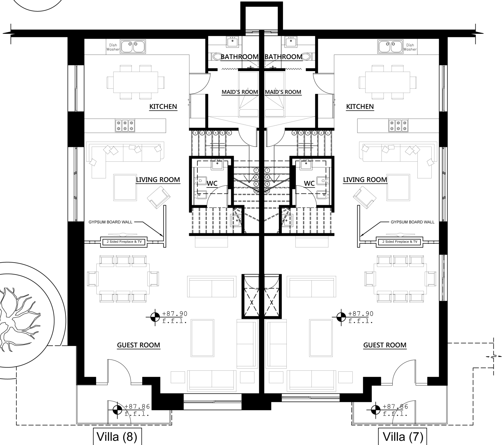
GROUND FLOOR PLAN - VILLA 7&8 BUILDING (A)
